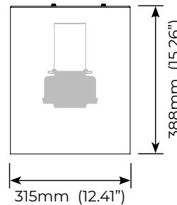
13" Cylinder Reflector shown with VA6 Lamp
